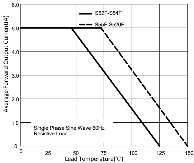
FIG1: Io-TL Curve
